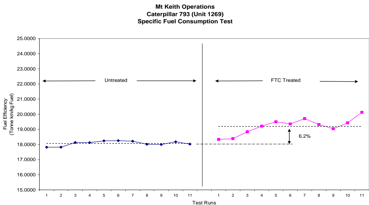
Figure 2 Typical results of specific fuel consumption tests at MKO
